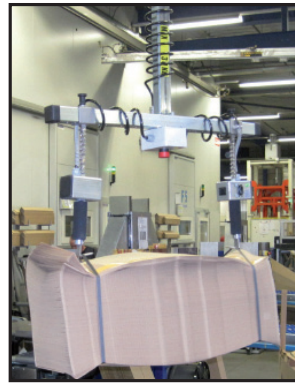
Tool for lifting bundles of paper sacks
