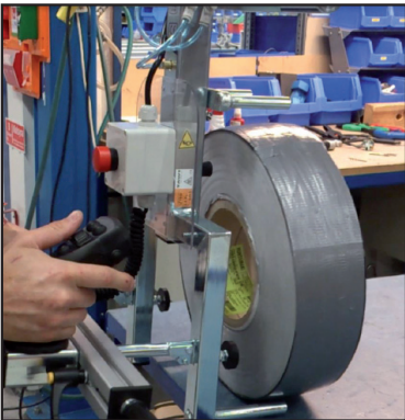
Roll handling pneumatic gripper, paper roll with adjustable joystick control
